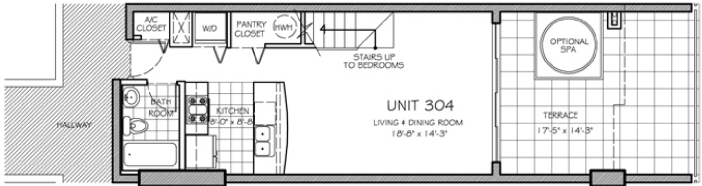
ENTRANCE LEVEL
