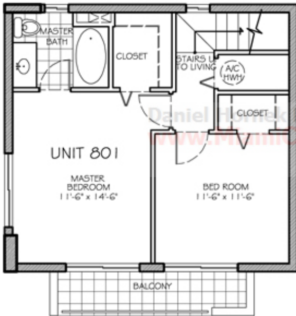
LOWER LEVEL
