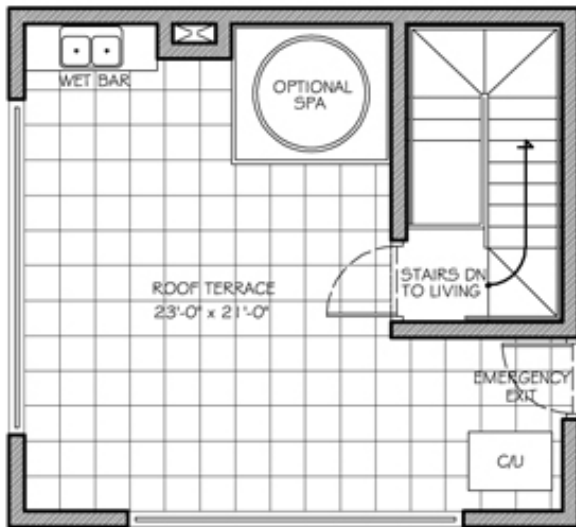
ROOF TERRACE
